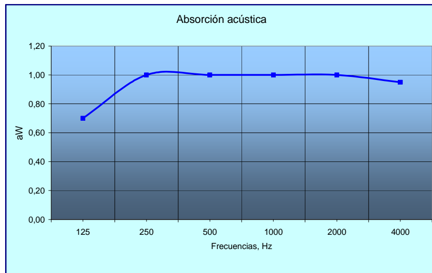
Class A, \alpha_w = 1,0 ISO 11654; method ISO 354 E=200
