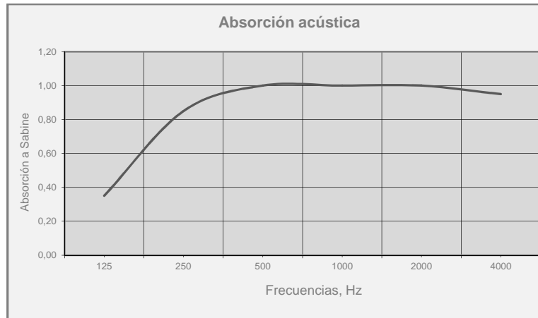
RONDA CONCEPT Class A, ( \alpha_w = 0,95 ) ISO 11654; method ISO 354 E=200
