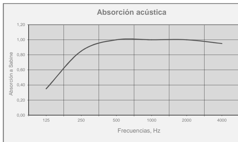
TALOS 30, 60, 100 Class A, ( \alpha_w = 0,95 ) ISO 11654; method ISO 354 E=200
